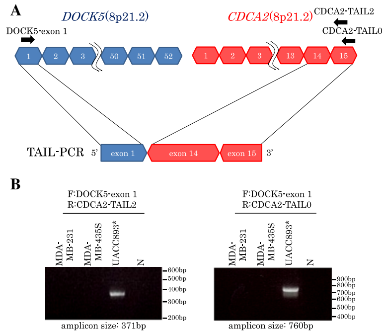
Figure 11 TAIL-PCR detection and RT-PCR confirmation of fusion gene DOCK5-CDCA2 . Acquired fusion fragments by TAIL-PCR and exon structures of fusion partners are shown in (A) Red blocks are exons of candidate gene, blue blocks are exons of detected genes by TAIL-PCR. Arrows are primers for RT-PCR. RT-PCR confirmations for indicated samples are shown in (B) F: forward primer, R: reverse primer, *: detected samples in the program.
